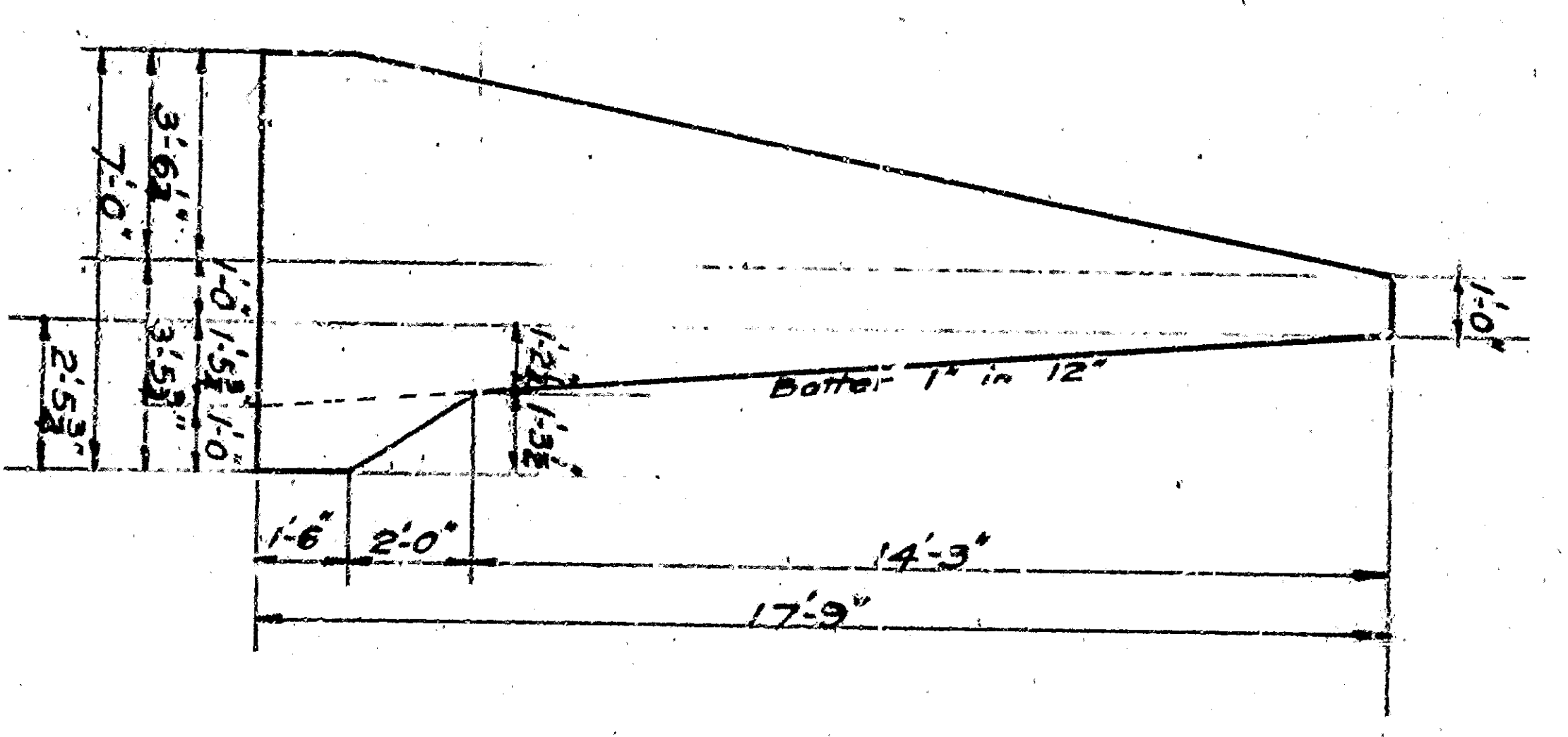
SECTION B-B
